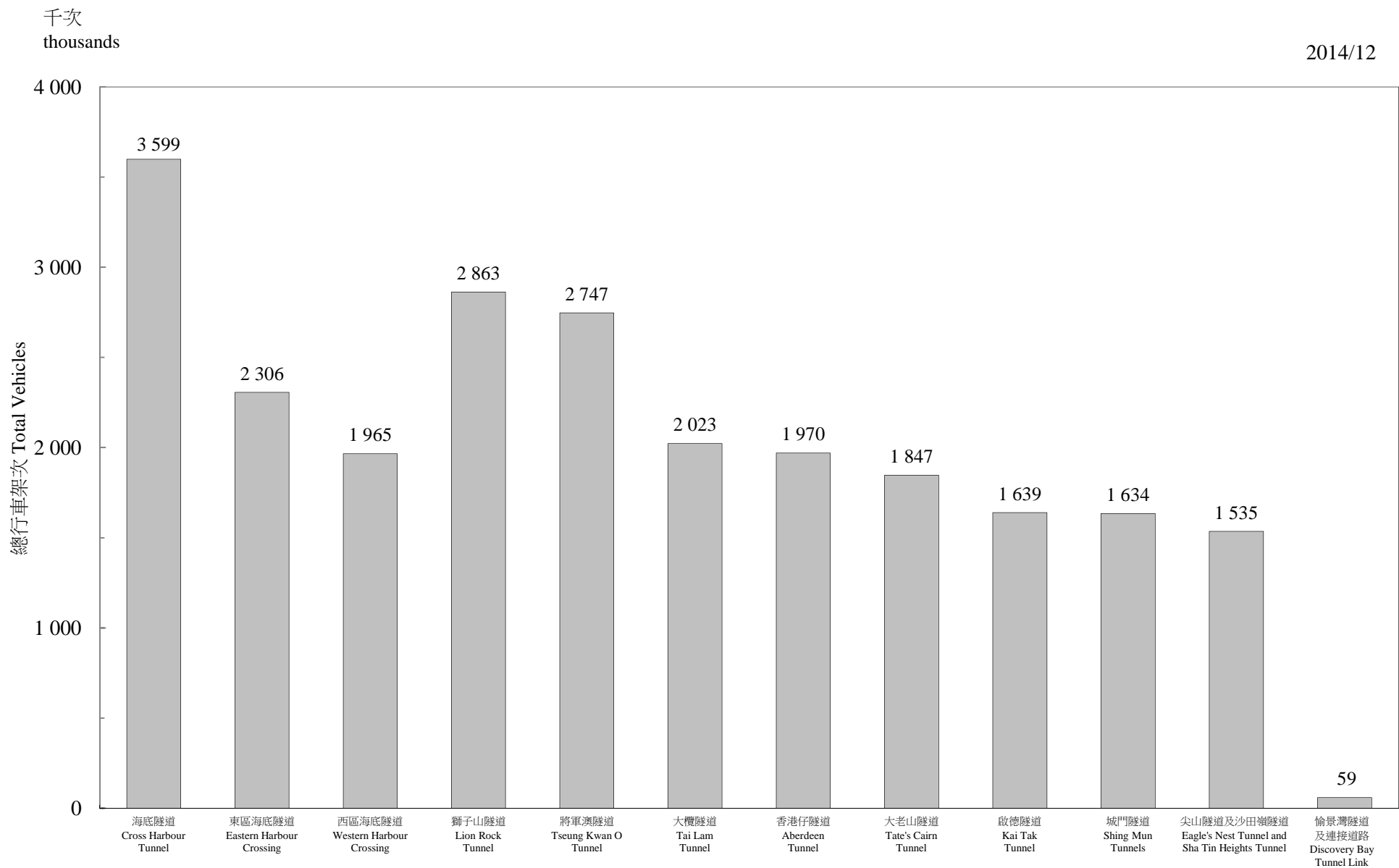
圖 3.1 - 隧道汽車流量 (二零一四年十二月) Chart 3.1 - Vehicular Flow Through Tunnels (December 2014)
